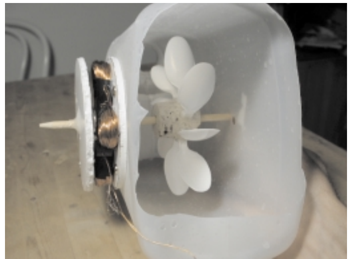
The completed micro-hydro turbine.
