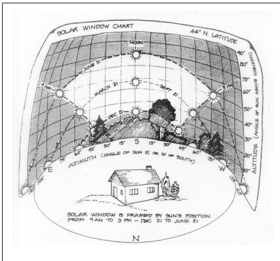
Illustration 2. The Solar Window. (Illustration courtesy of the Wisconsin Energy Bureau)
